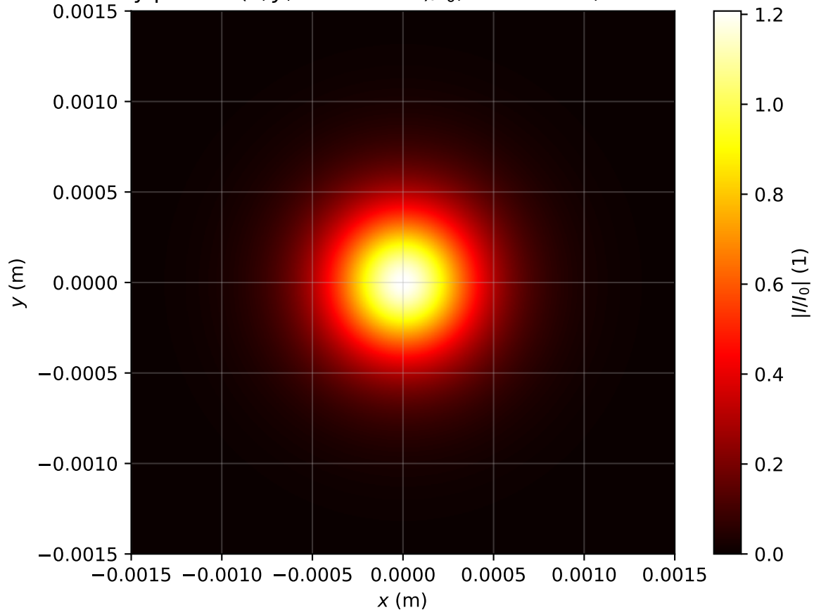
Intensity profile I(x, y, z = 1.353m)/I_0 , P_{in}=0.7P_{cr} , artificial time
